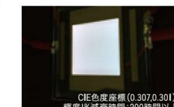
Tandem-type organic white-light EL device using yellow-emitting TADF material and blue material
